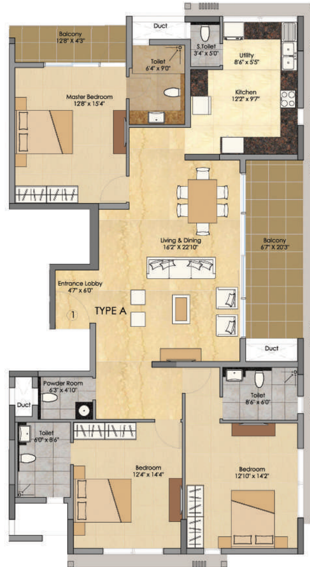
UNIT A SUPER BUILT UP AREA - 220 Sqm / 2372 Sft CARPET AREA - 142 Sqm / 1523 Sft
